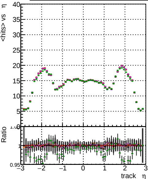
mean hits vs \eta Legend: - BOW original original vector 1000evt - BOW fitted 1000evt - BOW fit cpeok SORTRZZ 1000evt - BOW fit cpeok SORTRZZ TESTOUTLIER3 1000evt
