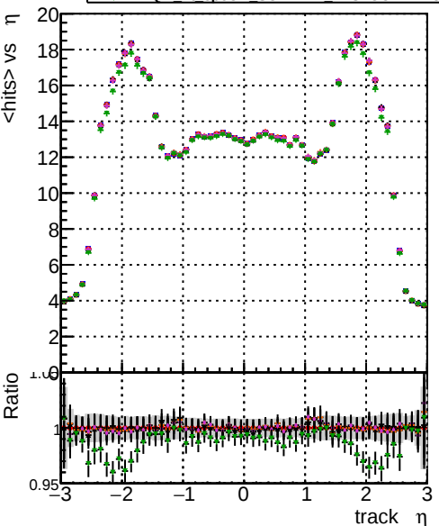
mean hit \eta Legend: BQM original original vector 1000evt, BQM fitted 4 1000evt, BQM fitted 22 1000evt, BQM fitted 22 1000evt, BQM fitted 22 1000evt, BQM fitted 22 1000evt
