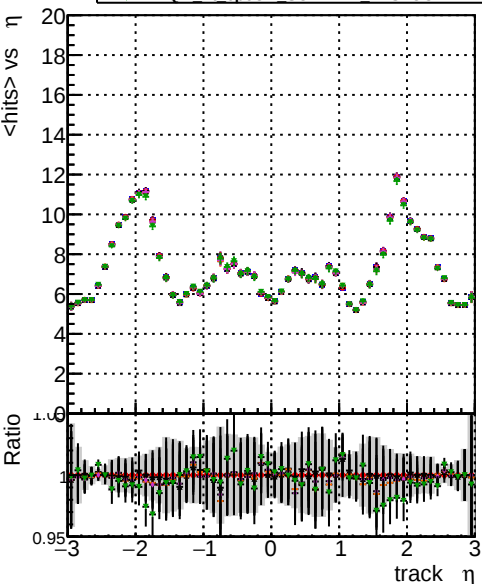
mean hits vs \eta Legend: - BOW original original vector 1000evt - BOW fitted 4 1000evt - BOW fit cpeok SORTZZ 1000evt - BOW fit cpeok SORTZZ TESTOUTLIER3 1000evt
