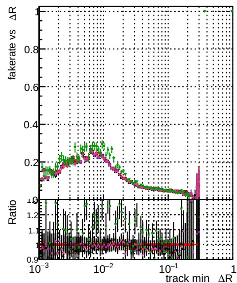
Fake rate vs \Delta R(\text{track, jet}) for DOM, original, originalvector, 1000evt, 10000evt, 100000evt, 1000000evt, QM, IL, EDEK, SORTRZ2, TESTOUTLIER2, 1000evt
