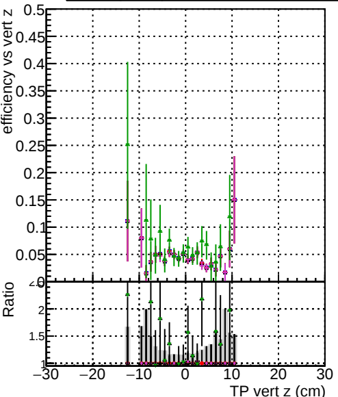
Efficiency vs vertpos Legend: BQM original original vector 1000evt BQM fitted 1000evt BQM fitted 4 1000evt BQM fitted cpeok SORTRZZ 1000evt BQM fitted TESTOUTLIER2 1000evt
