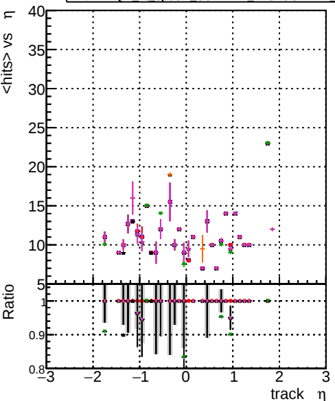
mean hits vs \eta Legend: - BOW original vector 1000evt - BOW fitted 1000evt - BOW fit cpeok SORTRZZ 1000evt - BOW fit cpeok SORTRZZ TESTOUTLIER 1000evt
