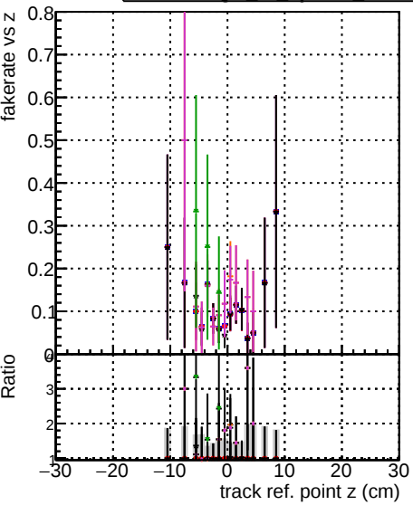
Fake rate vs v DOM original, original vector, 1000evt, 10000evt, 100000evt, DOM III CDEC SORTRZ2 1000evt
