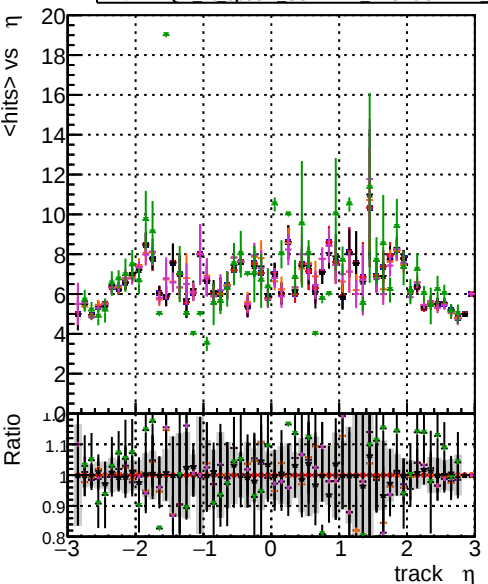
mean hits vs \eta Legend: BQM original vector 1000evt, BQM fitted 1000evt, BQM hit cpeok SORTRZZ 1000evt, BQM hit cpeok SORTRZZ TESTOUTLIER 1000evt
