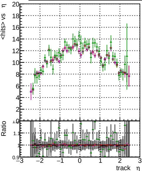
mean hits vs \eta Legend: BGM original, BGM fitted, BGM cpeok, BGM SORTRZZ, TESTOUTLIER
