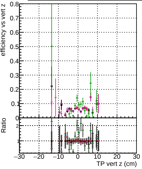
Efficiency vs vertpos Legend: original original vector fitted 4 cpeok SORTRZZ TESTOUTLIER
