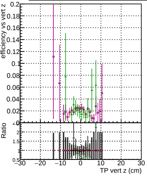
Efficiency vs vertpos Legend: original fitted cpeok SORTRZZ TESTOUTLIER
