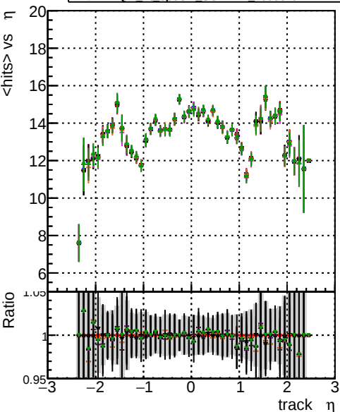
mean hits vs \eta Legend: - BOW original original vector 1000evt (blue) - BOW fitted 4 1000evt (red) - BOW fit no cut 1000evt (green) - BOW fit cpeok SORTZ 1000evt (orange) - BOW fit cpeok SORTZ 1000evt (purple) - BOW fit cpeok SORTZ 1000evt (pink) - BOW fit cpeok SORTZ 1000evt (light green)
