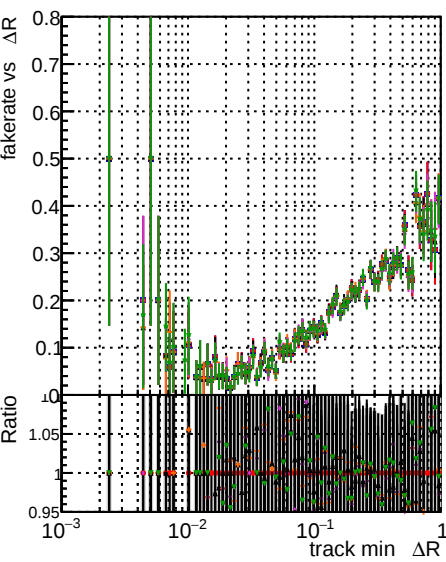
Fake rate vs \Delta R(\text{track, jet}) 1000evt
