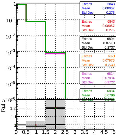
mean hits vs \eta Legend: - blue line: BGM original original vector 1000evt - red line: BGM fitted 1000evt - green line: BGM fit no cut 1000evt - orange line: BGM fit cpeok SORTRZ 1000evt
