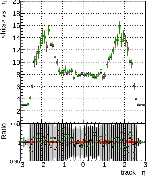
mean hits vs \eta Legend: - blue line: BGM original original vector 1000evt - red line: BGM fitted 1000evt - green line: BGM fit no cut 1000evt - orange line: BGM fit cpeok SORTRZ 1000evt
