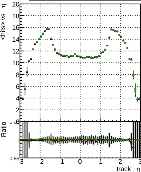
mean hits vs \eta Legend: - BOW original original vector 1000evt - BOW fitted 4 1000evt - BOW fit no cpe 1000evt - BOW fit cpeok SORTRZ 1000evt
