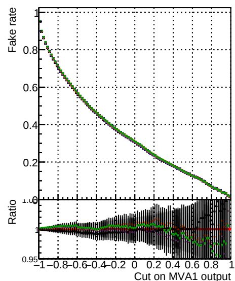
Fake rate vs. MVA1
