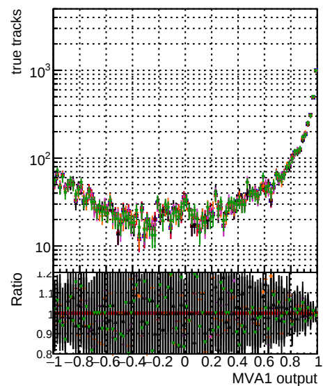
N of associated tracks (recoToSim) vs MVA1
