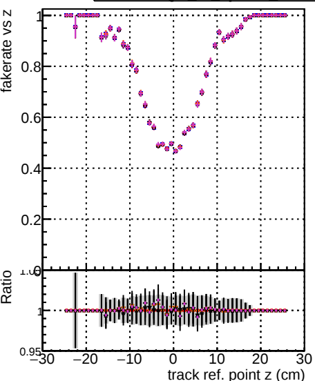
Fake rate vs verpos Legend: - Blue line: DOM original vector 1000evt - Red line: DOM hit peak 1000evt - Green line: DOM hit peak 1000evt - Purple line: DOM hit peak 1000evt
