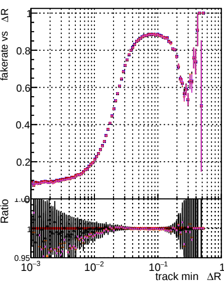
Fake rate vs \Delta R (track, jet) Legend: - DOM original 1000evt (blue line with dots) - DOM fit 1000evt (red line with dots) - DOM original 1000evt (green line with dots) - DOM fit 1000evt (orange line with dots) - DOM original 1000evt (purple line with dots) - DOM fit 1000evt (brown line with dots)
