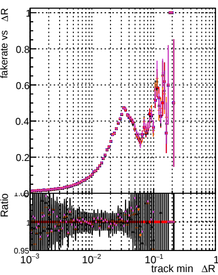
Fake rate vs \Delta R (track, jet) for different pileup levels and QCD hit checks.
