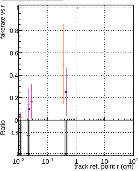
Fake rate vs v DOM original - original vector 1000evt DOM hit OK - hit OK 1000evt DOM hit OK 1000evt - hit OK 1000evt
