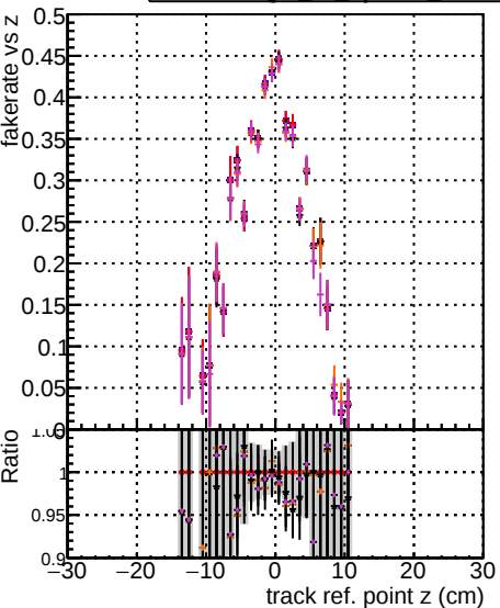
Fake rate vs v Legend: DOM original - original vector 1000evt DOM hit - hit 1000evt DOM hit - hit 1000evt DOM hit - hit 1000evt
