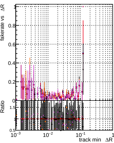
Fake rate vs \Delta R(\text{track, jet}) Legend: DOM original original vector 1000evt DOM hit 1000evt DOM hit 1000evt DOM hit 1000evt
