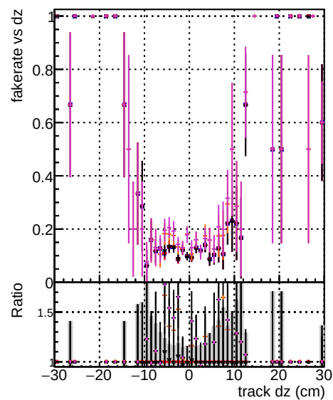
Fake rate vs d Legend: DOM original - originalvector_1000evt DOM original - originalvector_1000evt DOM original - originalvector_1000evt DOM original - originalvector_1000evt
