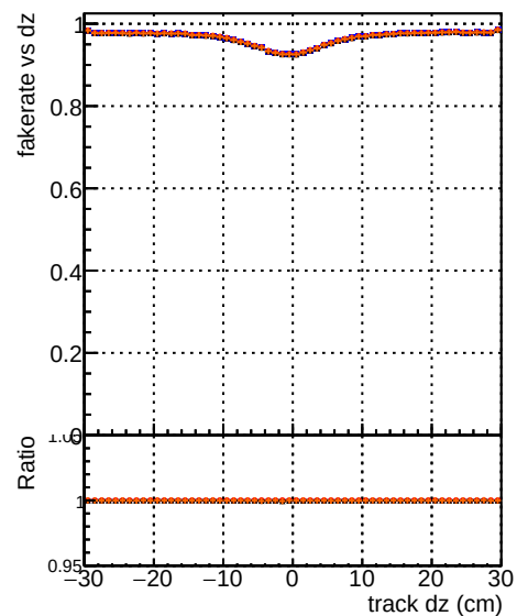
Fake rate vs dz Legend: DSM original - original vector 1000evt DSM original - original vector 10000evt DSM original - original vector 100000evt DSM original - original vector 1000000evt
