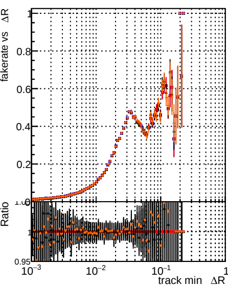
Fake rate vs \Delta R (track, jet) Legend: DOM original original vector 1000evt DOM fitted 1000evt DOM fit nocpe 1000evt
