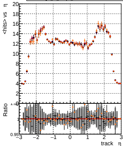
mean hits vs \eta Legend: - DQM_original_originalvector_1000evt (blue line with dots) - DQM_original_1000evt (red line with dots) - DQM_fitted4_1000evt (black line with dots) - DQM_fit_nocpe_1000evt (orange line with dots)
