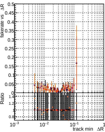
Fake rate vs \Delta R(\text{track, jet}) Legend: - DOM original 1000evt (blue line with dots) - DOM fitted 1000evt (red line with dots) - DOM hit nocpe 1000evt (black line with dots)
