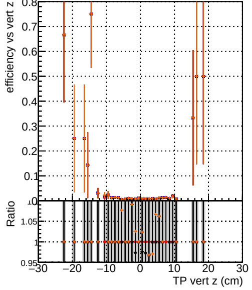
Efficiency vs vert z Legend: - DQM original originalvector_1000evt (blue line with circles) - DQM original_1000evt (red line with circles) - DQM fitted4_1000evt (black line with triangles) - DQM fit nocpe_1000evt (orange line with circles)
