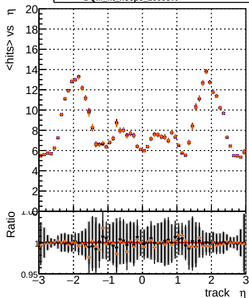
mean hits vs \eta Legend: DOM original originalvector_1000evt (blue line), DOM original_1000evt (red line), DOM fitted4_1000evt (black line), DOM fit nocpe_1000evt (orange line)
