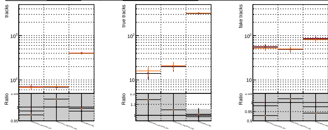
N of reco track vs. \chi^2 Legend: BGM original consistent BGM original BGM fit to the 1000 evts
