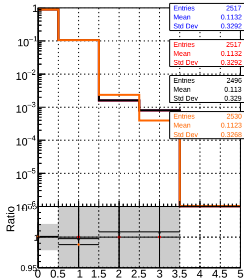
mean hits vs \eta Legend: DOM_original_originalvector_1000evt (blue line) DOM_original_1000evt (red line) DOM_fitted4_1000evt (black line) DOM_fit_nocpe_1000evt (orange line)
