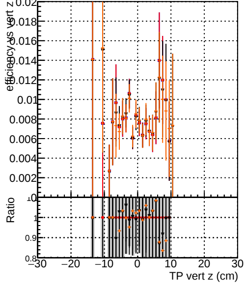
Efficiency vs. TP vert z (cm) Legend: - DOM_original_originalvector_1000evt (blue line with circles) - DOM_original_1000evt (red line with circles) - DOM_fitted4_1000evt (black line with circles) - DOM_fit_nocpe_1000evt (orange line with circles)
