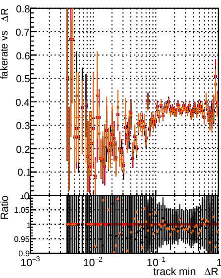
Fake rate vs \Delta R(\text{track, jet}) Legend: DOM original DOM fitted DOM hit DOM nocpe
