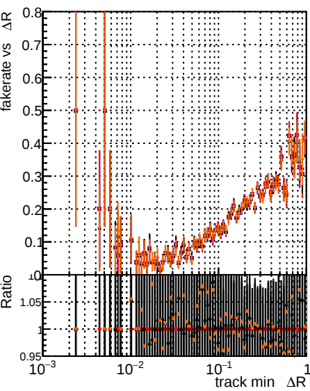
Fake rate vs \Delta R(\text{track, jet}) Legend: - blue line with dots: DOM original - red line with dots: DOM original vector 1000evt - black line with dots: DOM fitted 1000evt - orange line with dots: DOM fit nocpe 1000evt
