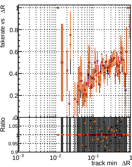
Fake rate vs \Delta R(\text{track, jet}) Legend: DOM original original vector 1000evt DOM fitted 1000evt DOM fit nocpe 1000evt
