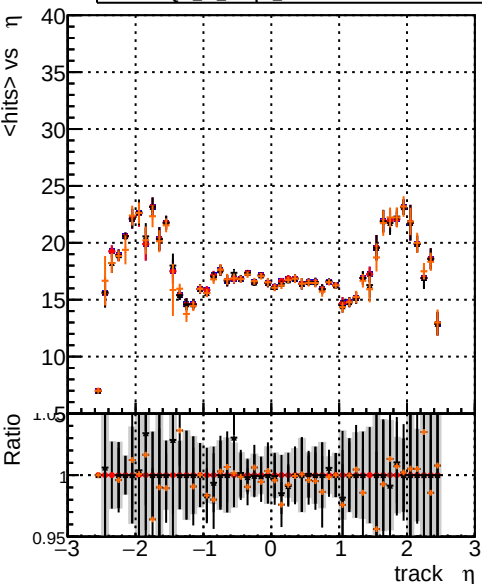
mean hits vs \eta Legend: DOM_original_originalvector_1000evt (blue line) DOM_original_1000evt (red line with error bars) DOM_fitted4_1000evt (black line with error bars) DOM_fit_nocpe_1000evt (orange line with error bars)
