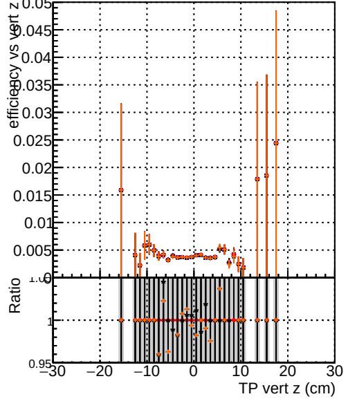
Efficiency vs vert z Legend: - DOM original originalvector_1000evt (blue line with circles) - DOM original_1000evt (red line with circles) - DOM fitted4_1000evt (black line with triangles) - DOM fit nocpe_1000evt (orange line with circles)
