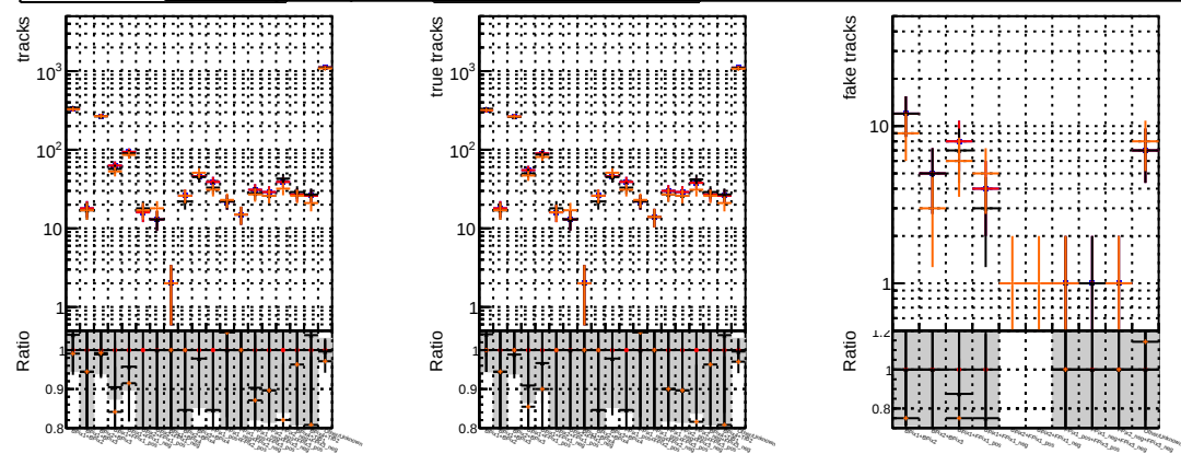
N of reco track vs. \chi^2 BSM original vector 1000evt BSM fit to the 1000evt
