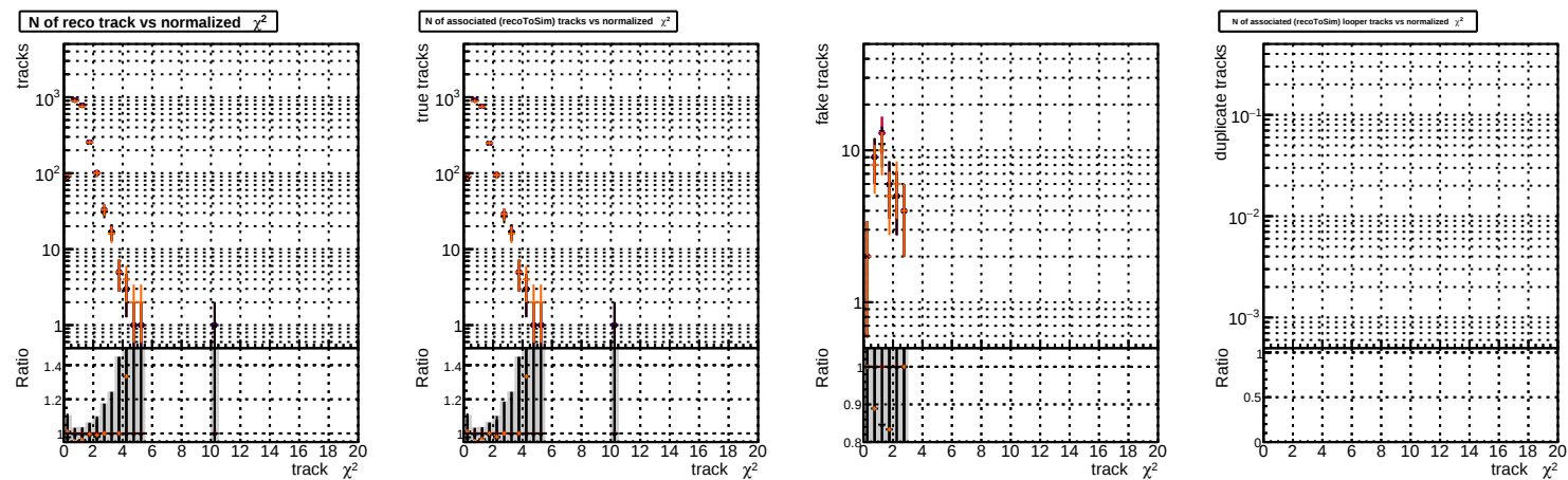
N of reco track vs. \chi^2 BSM original vector 1000evt BSM fit to the 1000evt
