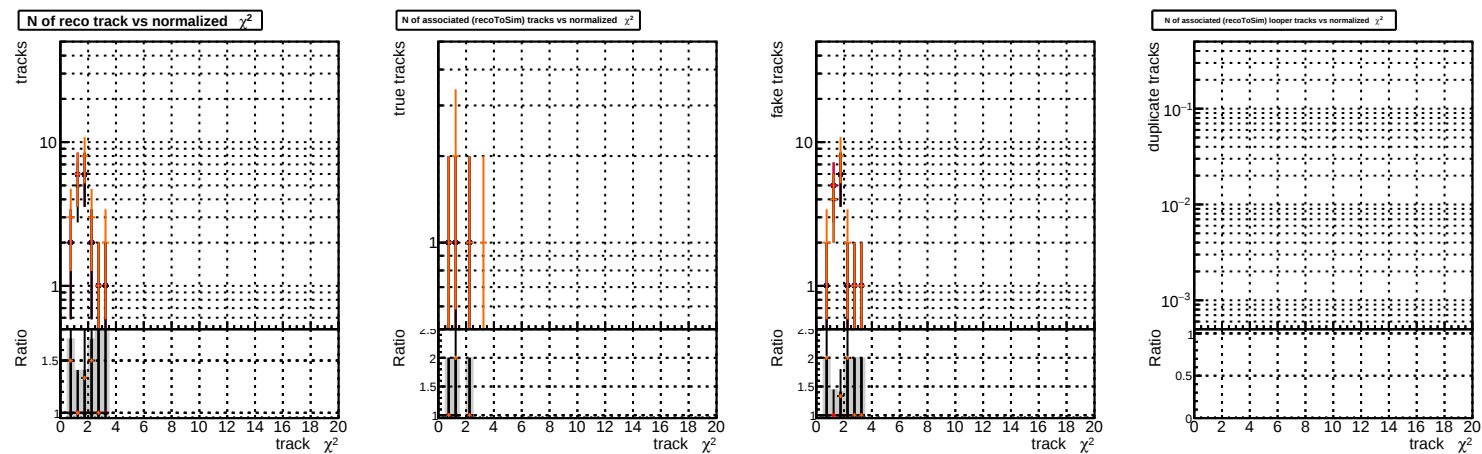
N of reco track vs. \chi^2 BSM original signal vector 1000evt BSM original signal vector 1000evt BSM fit to the 1000evt
