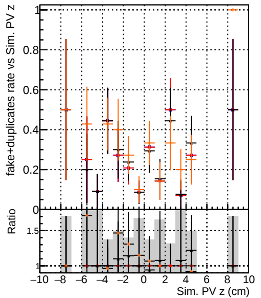
fake+duplicates rate vs Sim. PV z
