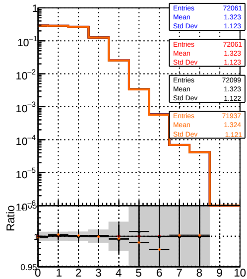
mean hits vs \eta Legend: DOM_original_originalvector_1000evt (blue line) DOM_original_1000evt (red line) DOM_fitted4_1000evt (black line) DOM_fit_nocpe_1000evt (orange line)
