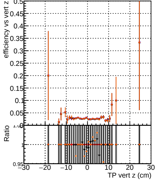
Efficiency vs vert z Legend: - DOM_original_originalvector_1000evt (blue line with circles) - DOM_original_1000evt (red line with circles) - DOM_fitted4_1000evt (black line with circles) - DOM_fit_nocpe_1000evt (orange line with circles)
