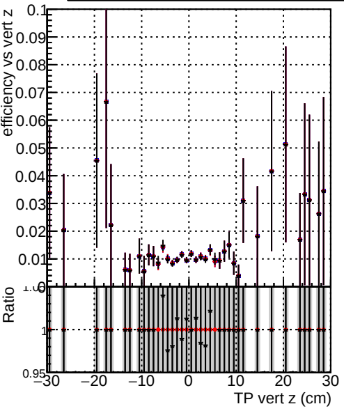
Efficiency vs vert z Legend: DQM_original_originalvector_1000evt (blue line with circles) DQM_original_1000evt (red line with circles) DQM_fitted4_1000evt (black line with circles)
