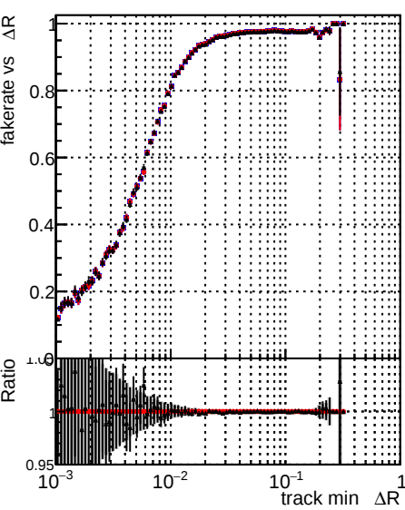
Fake rate vs \Delta R(\text{track, jet}) Legend: DQM original originalvector_1000evt (blue line with dots) DQM original 1000evt (red line with dots) DQM fitted4 1000evt (black line with dots)
