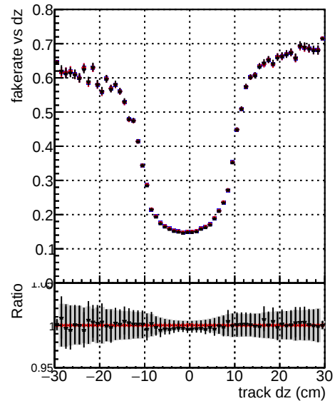
Fake rate vs dz — DOM original — original vector — DOM fitted — original 1000evt — DOM fitted 1000evt
