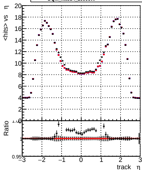
mean hits vs \eta Legend: DQM_original_originalvector_1000evt (blue line), DQM_original_1000evt (red line), DQM_fitted4_1000evt (black line)
