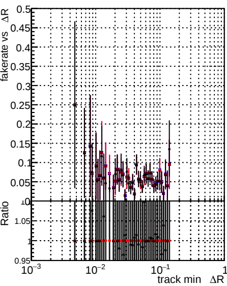
Fake rate vs \Delta R(\text{track, jet}) Legend: DQM original originalvector_1000evt (blue line with squares) DQM original_1000evt (red line with circles) DQM fitted4_1000evt (black line with crosses)
