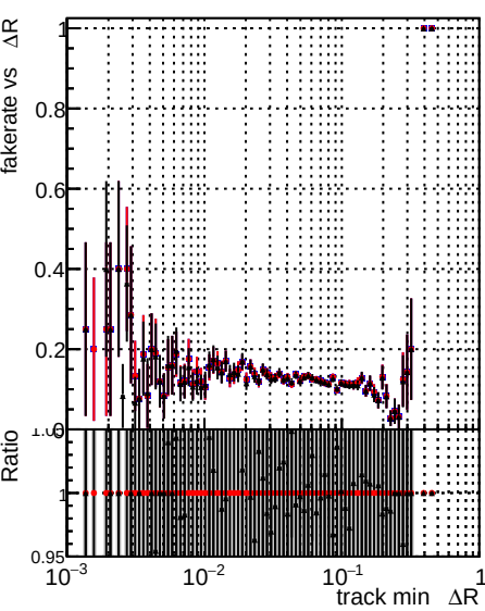
Legend: \Delta R(\text{track, jet}) \Delta R(\text{track, jet}) \Delta R(\text{track, jet})
