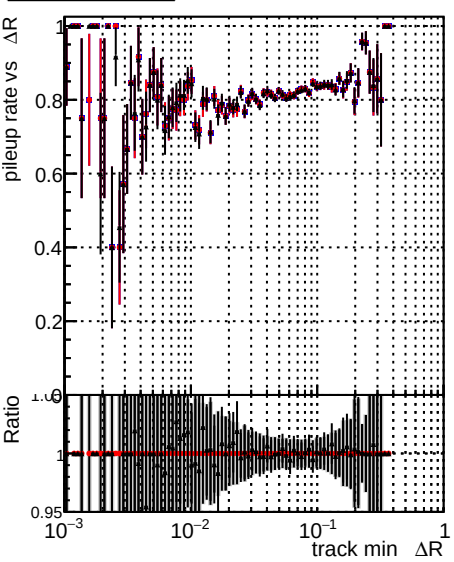
Legend: \Delta R(\text{track, jet}) \Delta R(\text{track, jet}) \Delta R(\text{track, jet})
