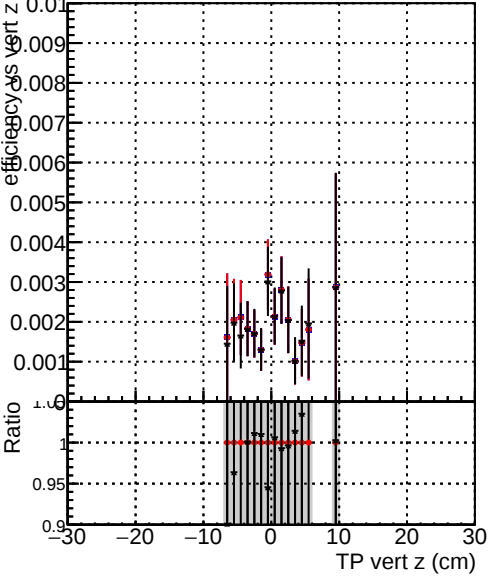
Efficiency vs TP vert z Legend: DQM_original_originalvector_1000evt (blue line with circles) DQM_original_1000evt (red line with circles) DQM_fitted4_1000evt (black line with circles)
