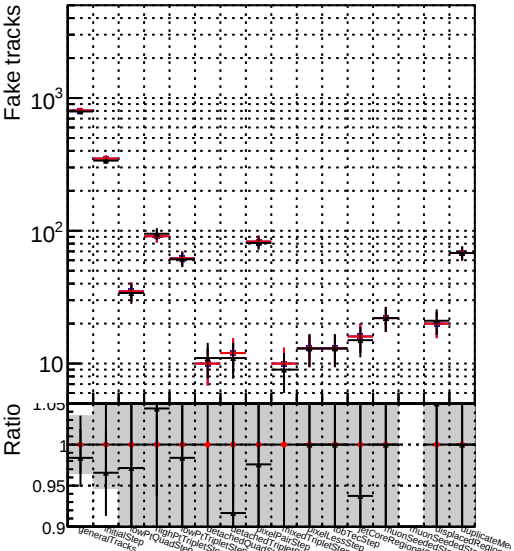
Number —●— DQM_original_1000ev —▲— DQM_fitted4_1000ev
